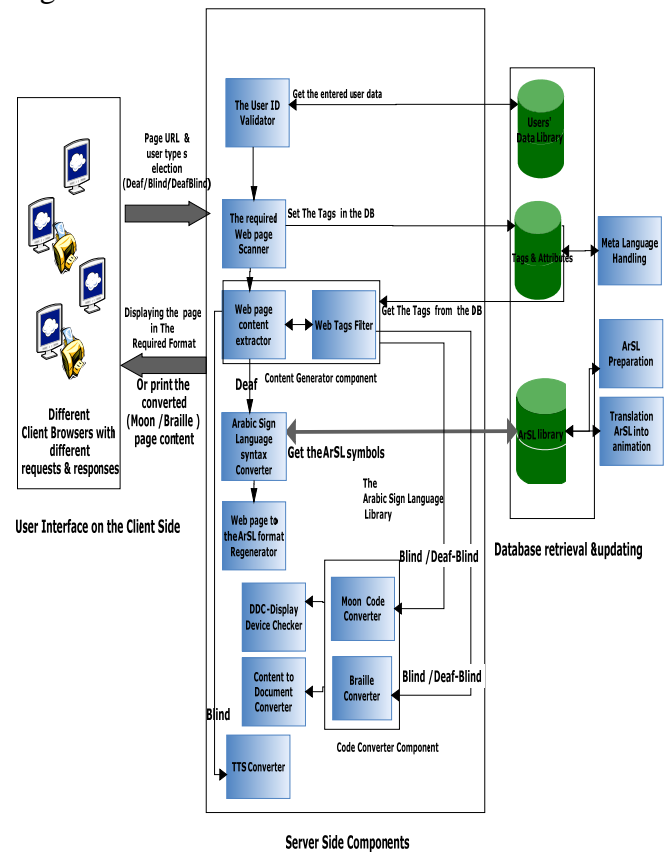
Fig. 2 The block diagram architecture of the proposed framework
