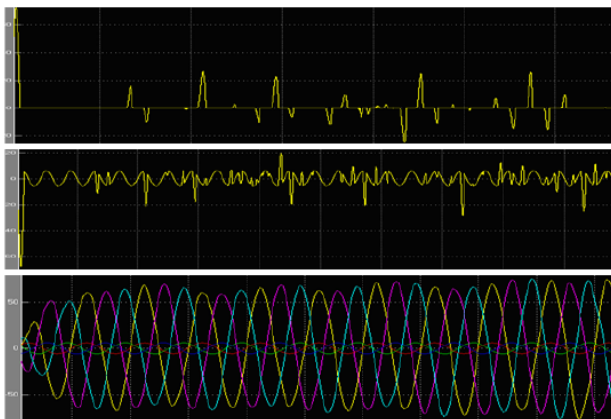
Fig. 9(b) Wave forms of load current, filter current, supply current and supply voltage of Unbalanced non linear load Using PI control with respect to time
