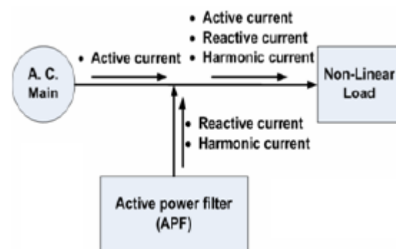
Fig. 1 Connection of shunt active filter with non-linear load
