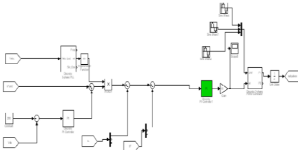
Fig. 6 Control strategy for shunt APF with PI-Controller
